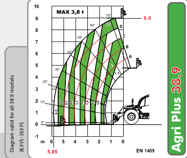
The measurements refer to the vehicle equipped with 405-70-24" tyres
