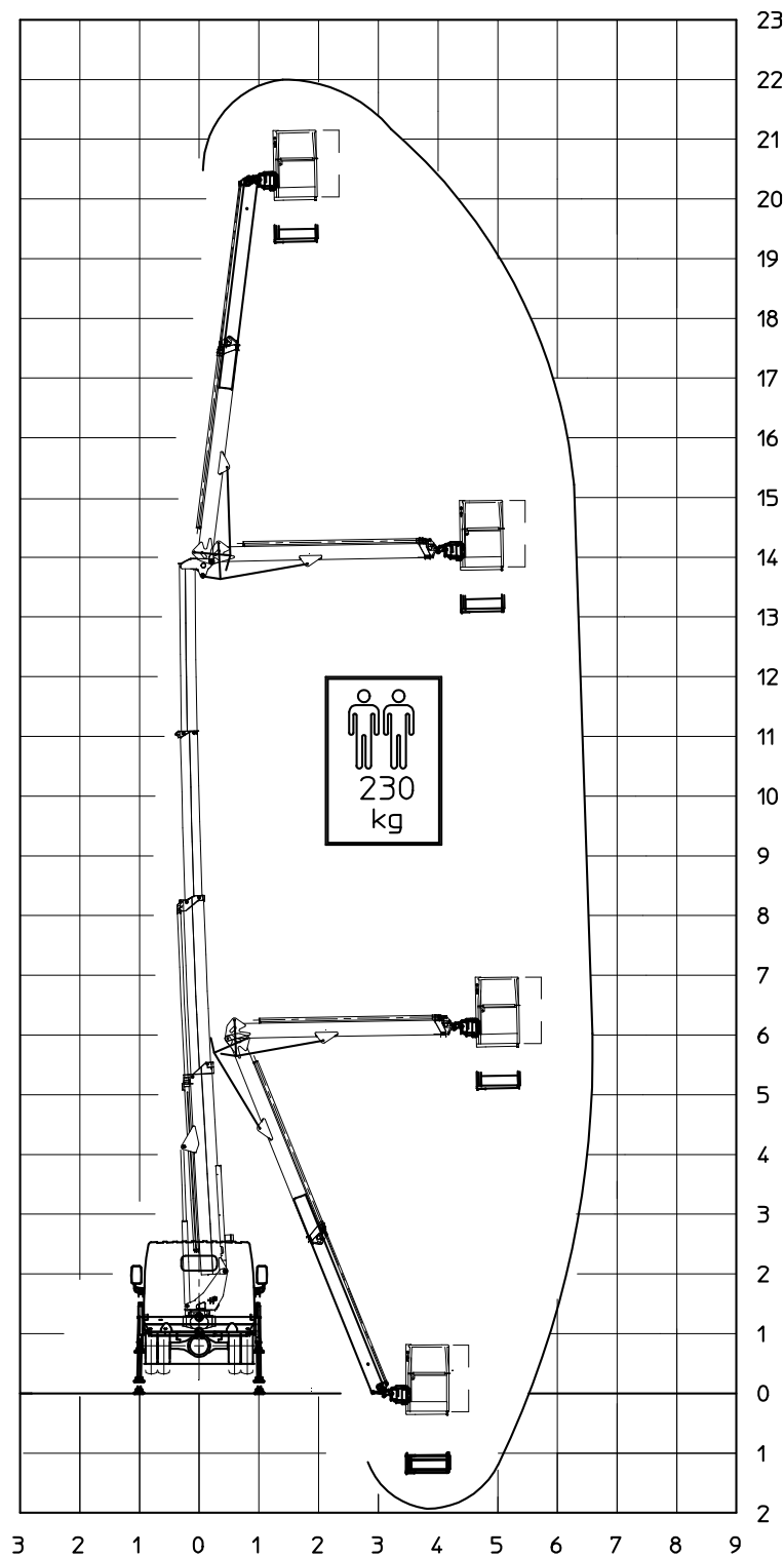
TRAVERSE IN SAGOMA - OUTRIGGER IN
