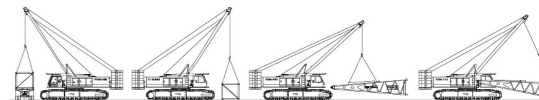
Unloading and assembling of boom
