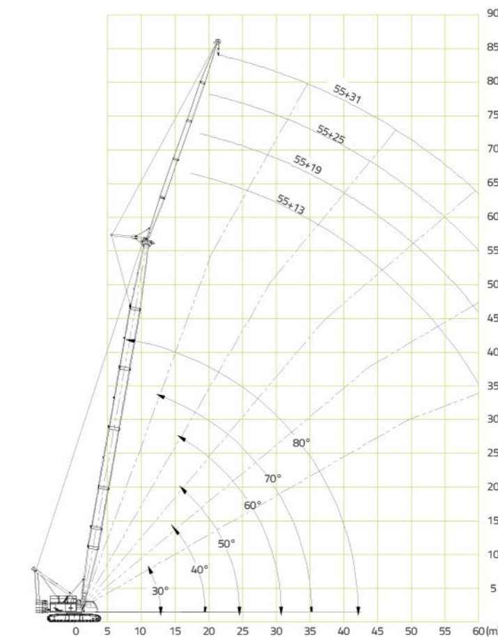
Main Boom + Fixed Jib Lifting Height Characteristics Curve (I) (SF Boom)
